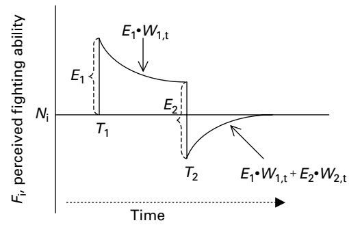
Fig. 2. Integration of experience effects for a naive individual i with an initial perceived fighting ability ( F_i ) of N_i . A winning experience at T_1 increases its perceived fighting ability by E_1 . This effect decays through time and W_{1,t} represents how the effect is weighted with the passage of time. A losing experience is added at T_2 and lowers individual i 's perceived fighting ability by |E_2| and the weighting function of this second experience is W_{2,t} . This combined effect gradually decays back to a perceived fighting ability of N_i .
