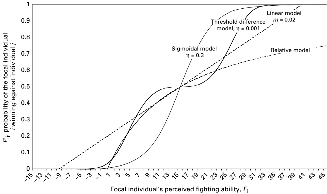
Fig. 3. Probability of winning ( P_{ij} ) predicted from the Linear [Section V (1), equation (2) with m arbitrarily set to 0.02], the Relative [Section V (1), equation (3)], the Sigmoidal [Section V (1), equation (4) with \eta arbitrarily set to 0.3], and the Threshold difference models [Section V (1), equation (5) with \eta arbitrarily set to 0.001] for a focal individual i with various perceived fighting ability ( F_i ) fighting against an opponent j with a perceived fighting ability ( F_j ) of 15.
